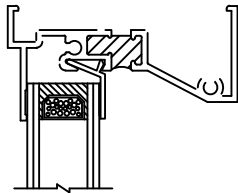
3/4" INSULATED GLASS
