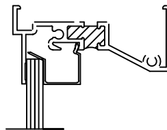
1/4" SINGLE GLASS
