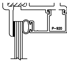
1/4" SINGLE GLAZED
