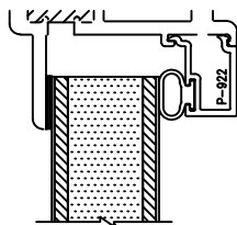
1" INSULATED PANEL
