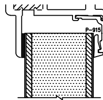
1 1/2" INSULATED PANEL
