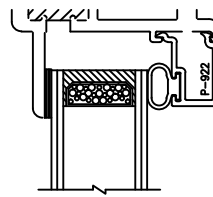
1" INSULATED GLASS
