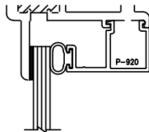
1/4" SINGLE GLAZED
