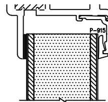
1 1/2" INSULATED PANEL
