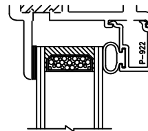
1" INSULATED GLASS
